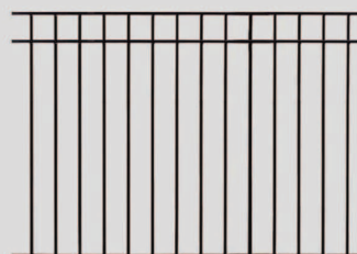
TPA5406R 54"x72-1/2" Pool Panel
